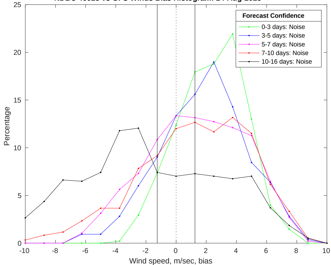
NDBC 46028 vs GFS Winds Bias Histogram: 24-Aug-2025
