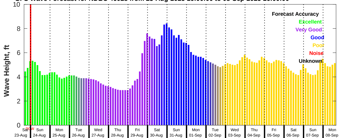
GFS Wave Forecast for NDBC 46028 from 23-Aug-2025 16:00:00 to 08-Sep-2025 16:00:00
