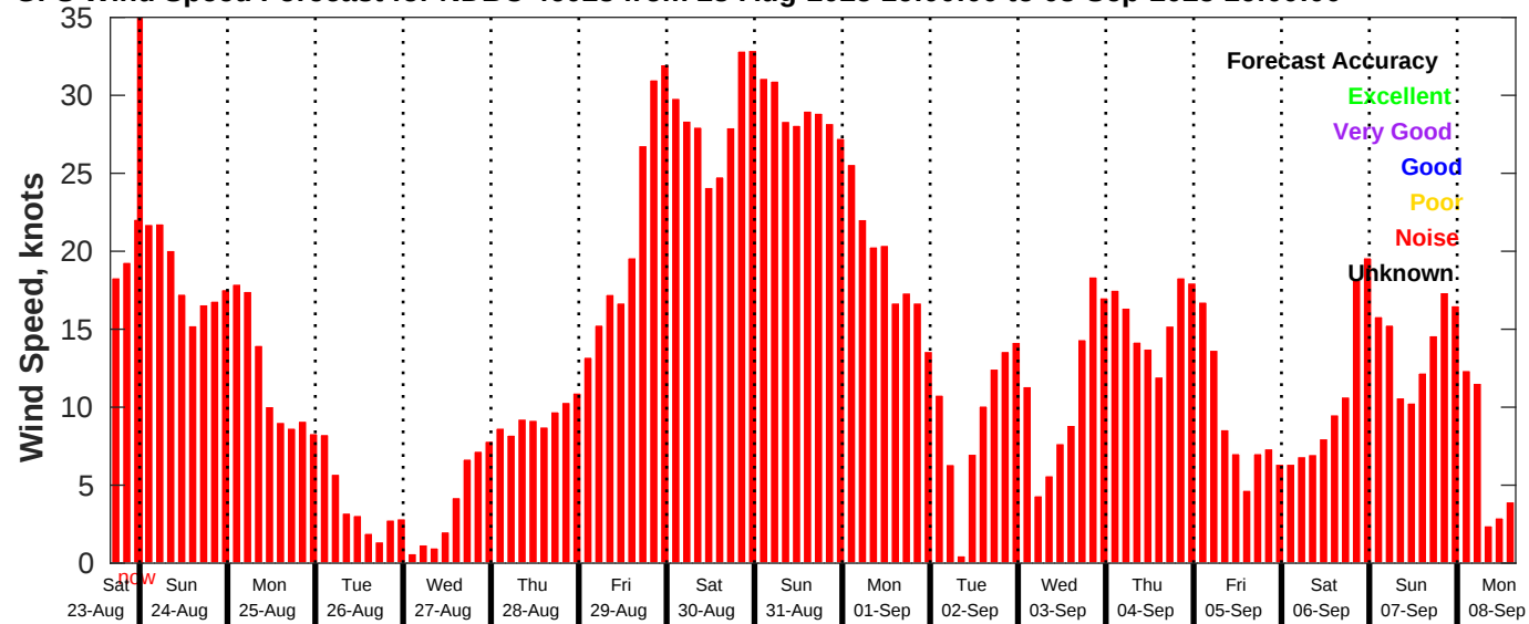
GFS Wind Speed Forecast for NDBC 46028 from 23-Aug-2025 16:00:00 to 08-Sep-2025 16:00:00
