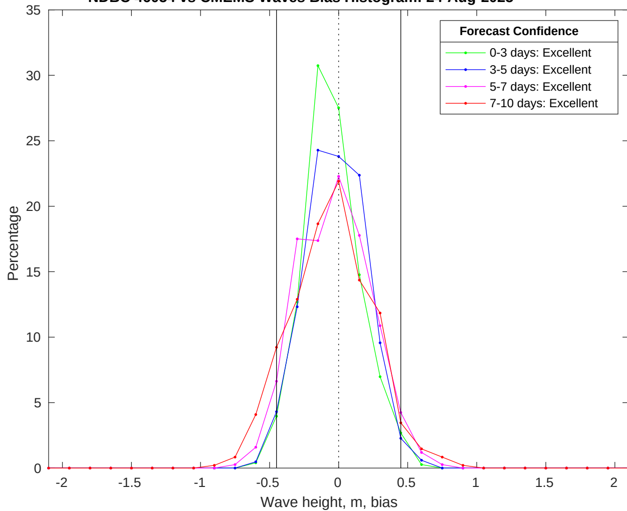
NDBC 46054 vs CMEMS Waves Bias Histogram: 24-Aug-2025
