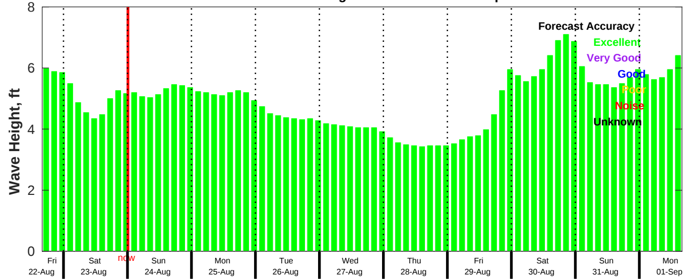
CMEMS Wave Forecast for NDBC 46054 from 22-Aug-2025 16:00:00 to 01-Sep-2025 16:00:00
