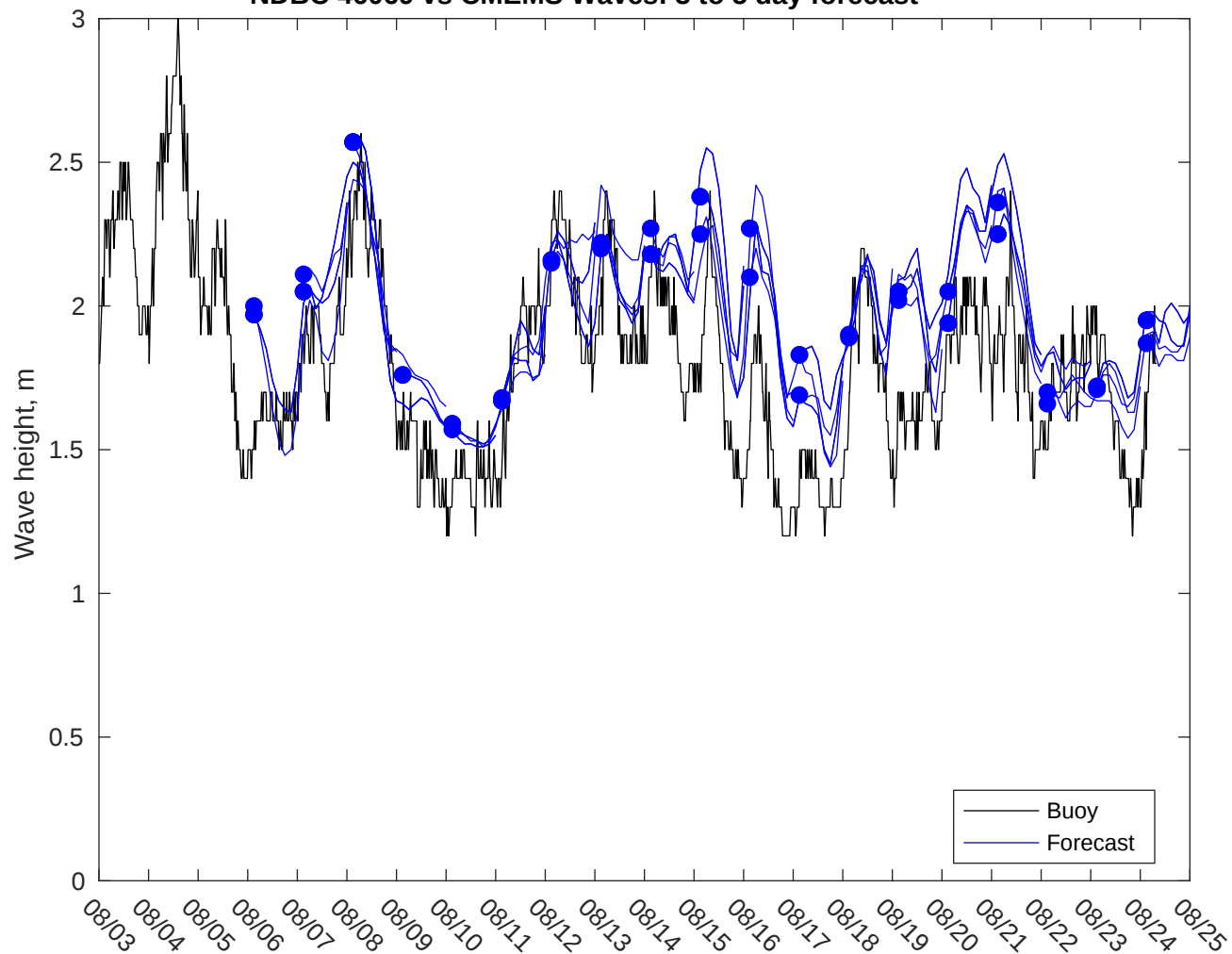
NDBC 46069 vs CMEMS Waves: 3 to 5 day forecast
