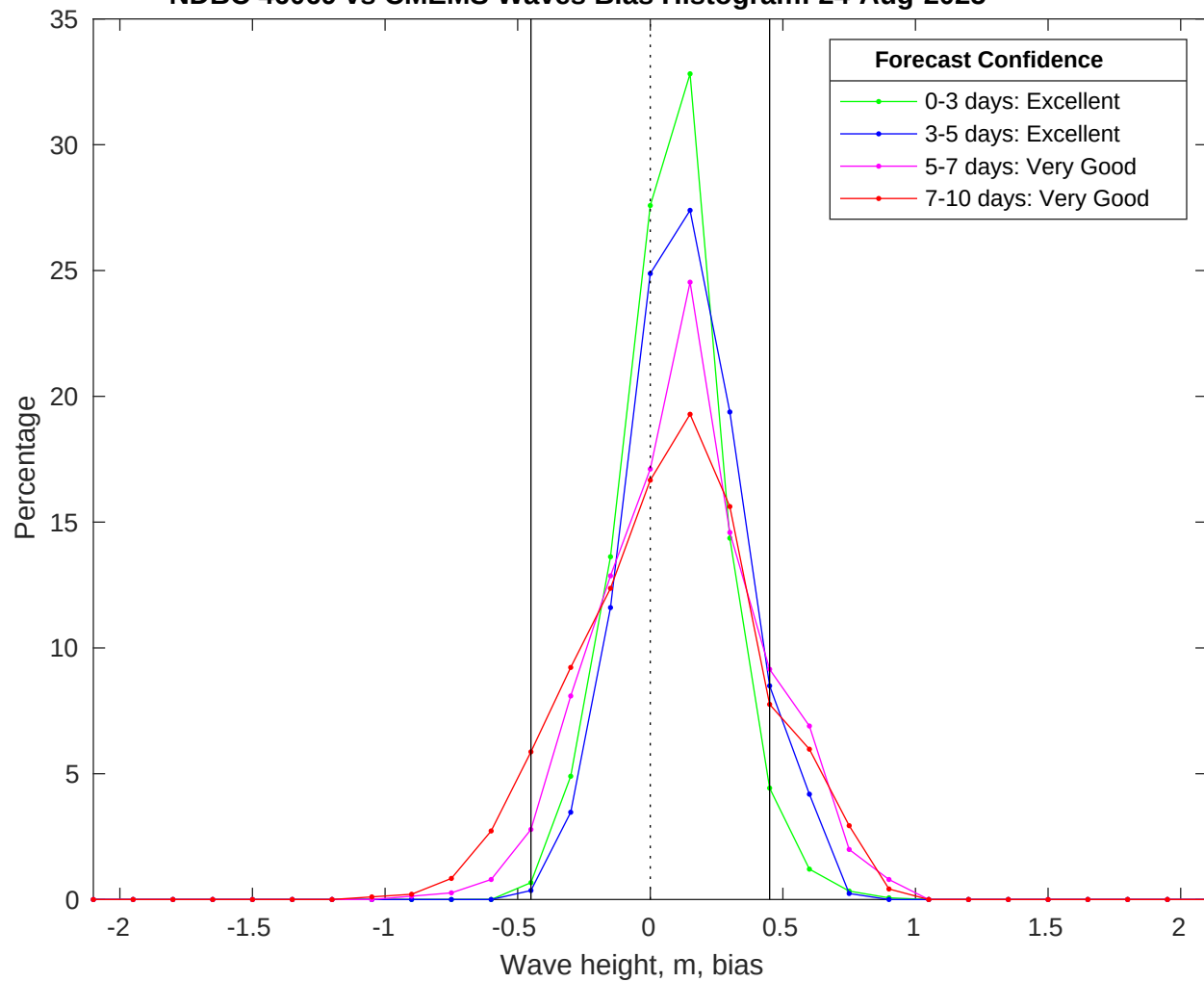
NDBC 46069 vs CMEMS Waves Bias Histogram: 24-Aug-2025
