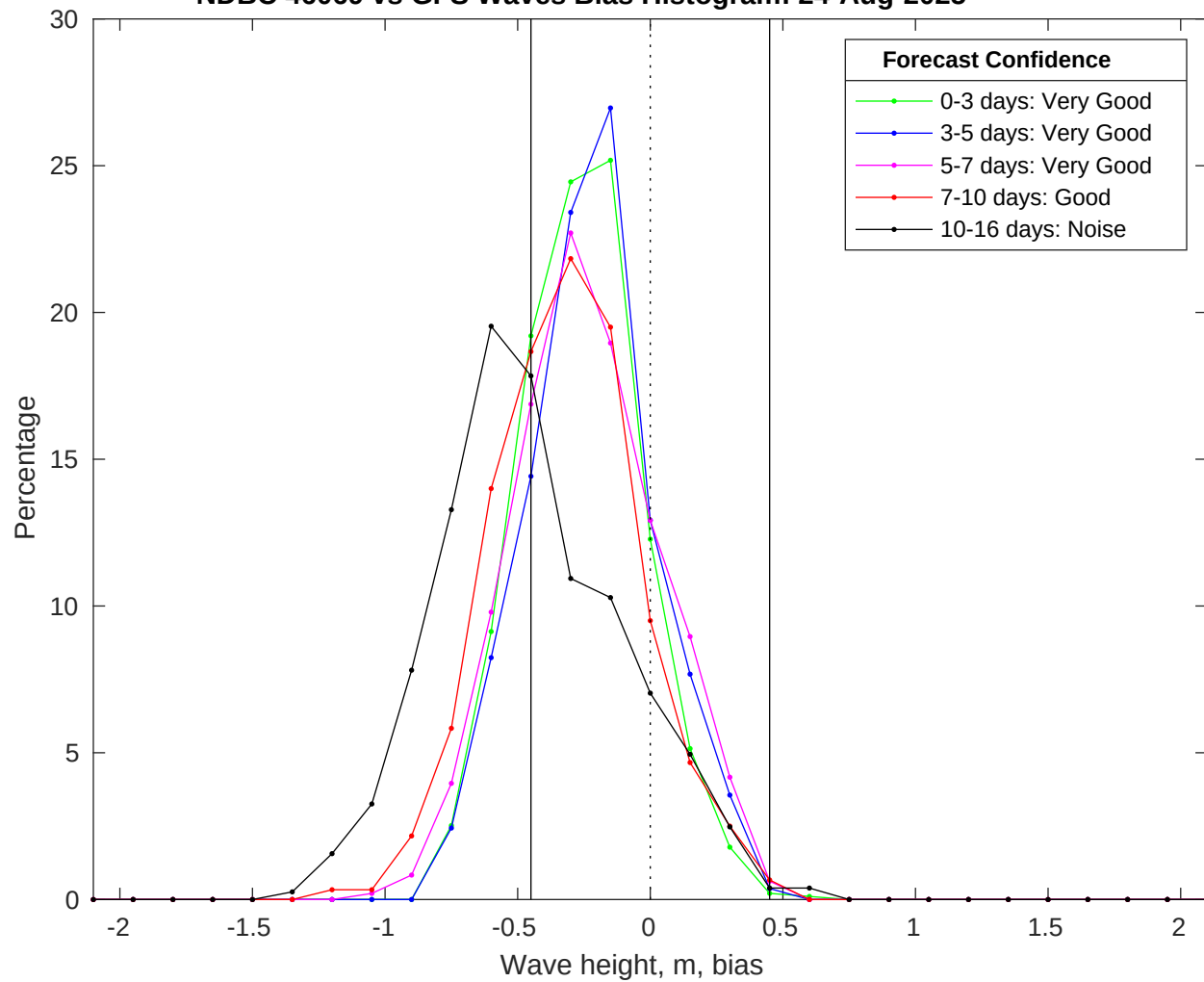
NDBC 46069 vs GFS Waves Bias Histogram: 24-Aug-2025
