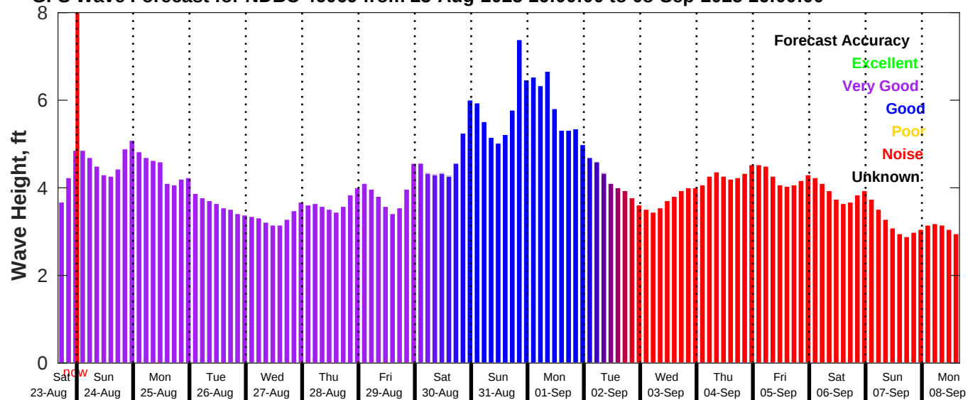
GFS Wave Forecast for NDBC 46069 from 23-Aug-2025 16:00:00 to 08-Sep-2025 16:00:00
