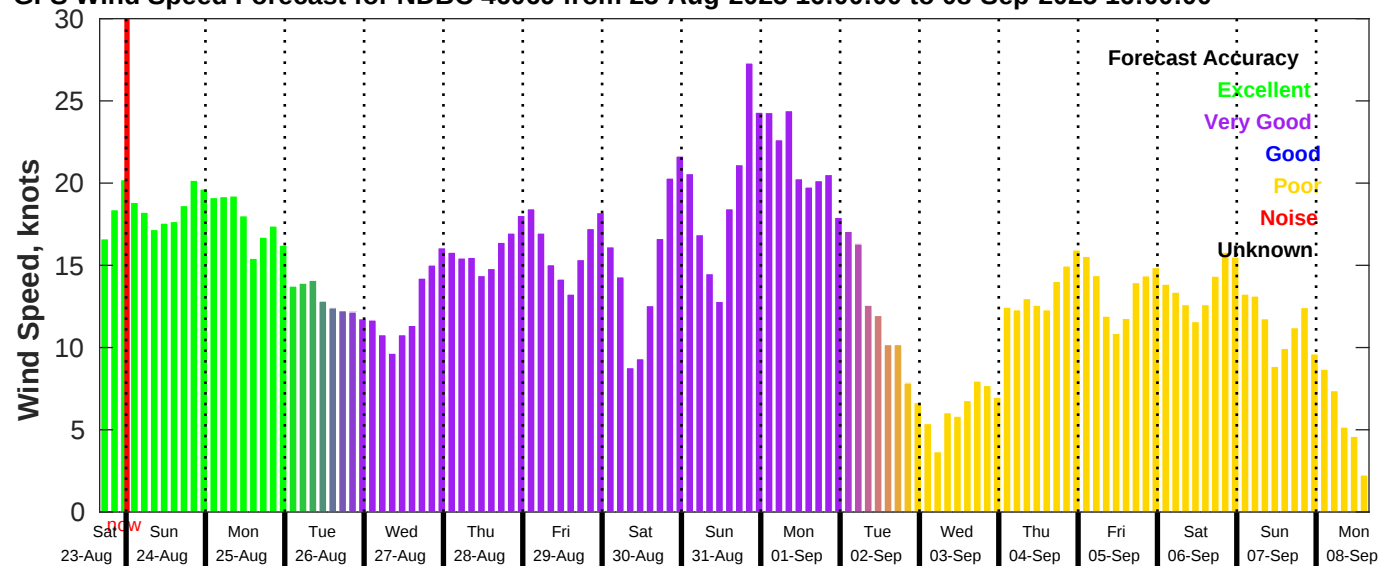
GFS Wind Speed Forecast for NDBC 46069 from 23-Aug-2025 16:00:00 to 08-Sep-2025 16:00:00
