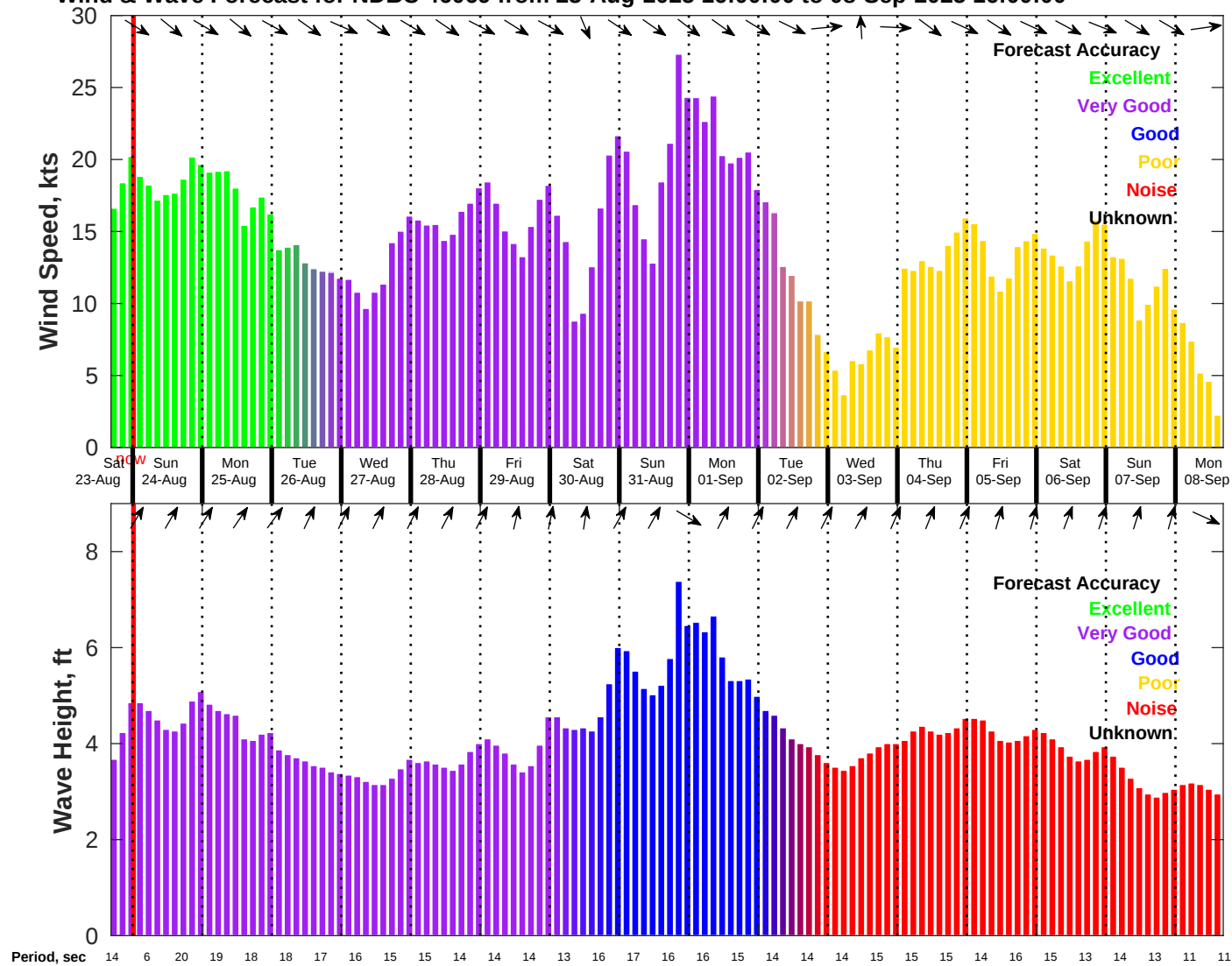
Wind & Wave Forecast for NDBC 46069 from 23-Aug-2025 16:00:00 to 08-Sep-2025 16:00:00
