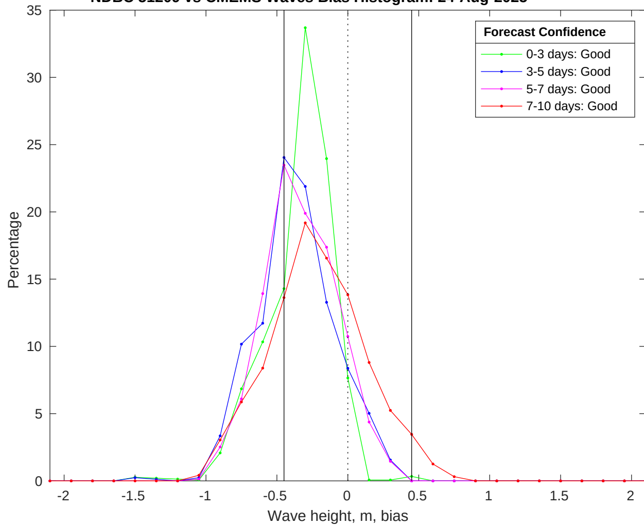
NDBC 51209 vs CMEMS Waves Bias Histogram: 24-Aug-2025
