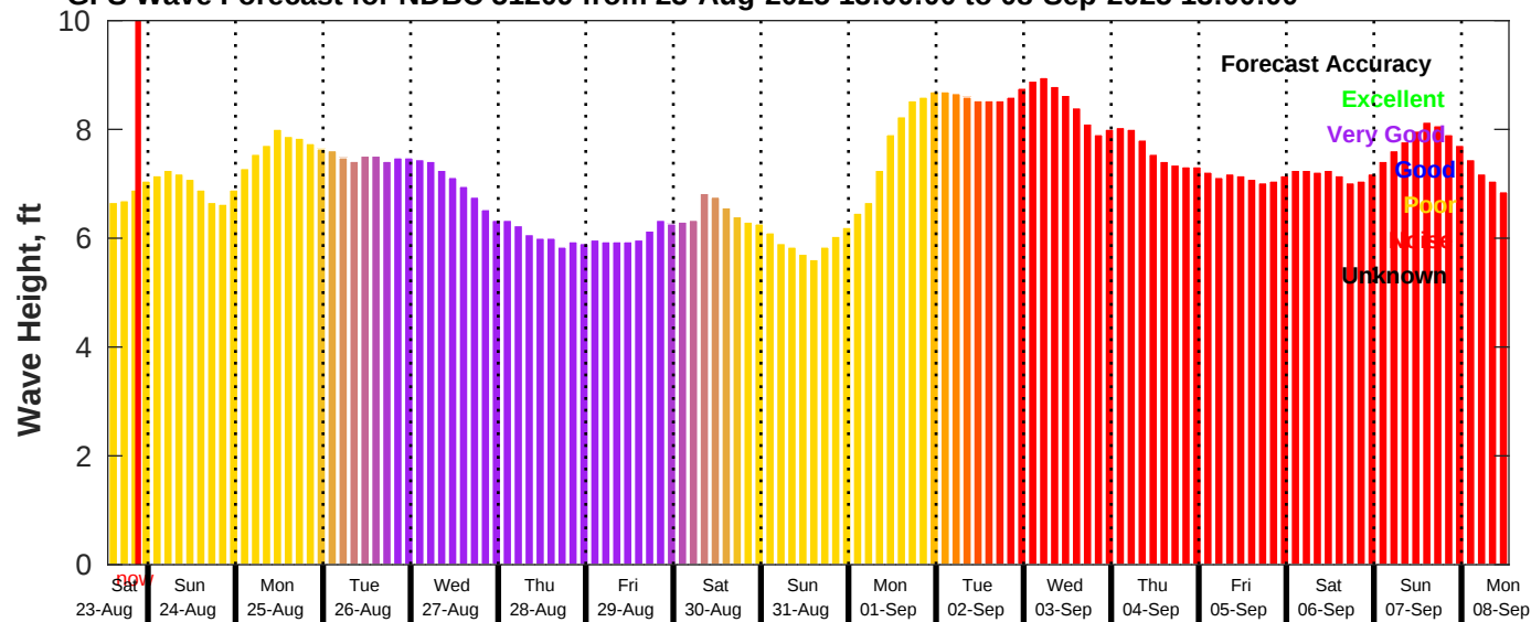
GFS Wave Forecast for NDBC 51209 from 23-Aug-2025 13:00:00 to 08-Sep-2025 13:00:00
