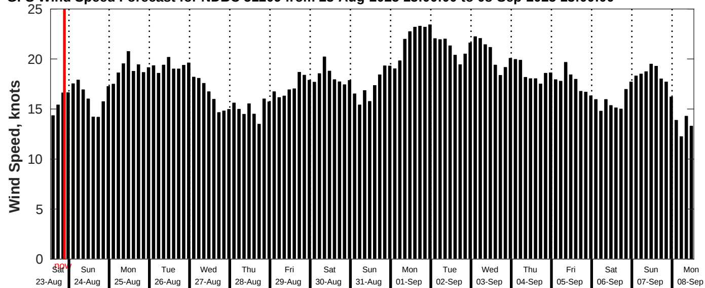
GFS Wind Speed Forecast for NDBC 51209 from 23-Aug-2025 13:00:00 to 08-Sep-2025 13:00:00
