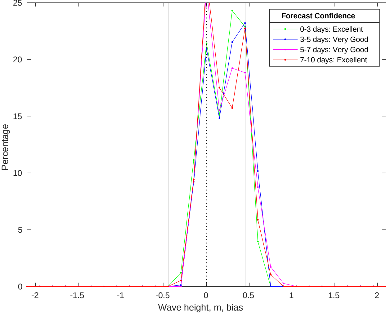
NDBC 51211 vs CMEMS Waves Bias Histogram: 24-Aug-2025
