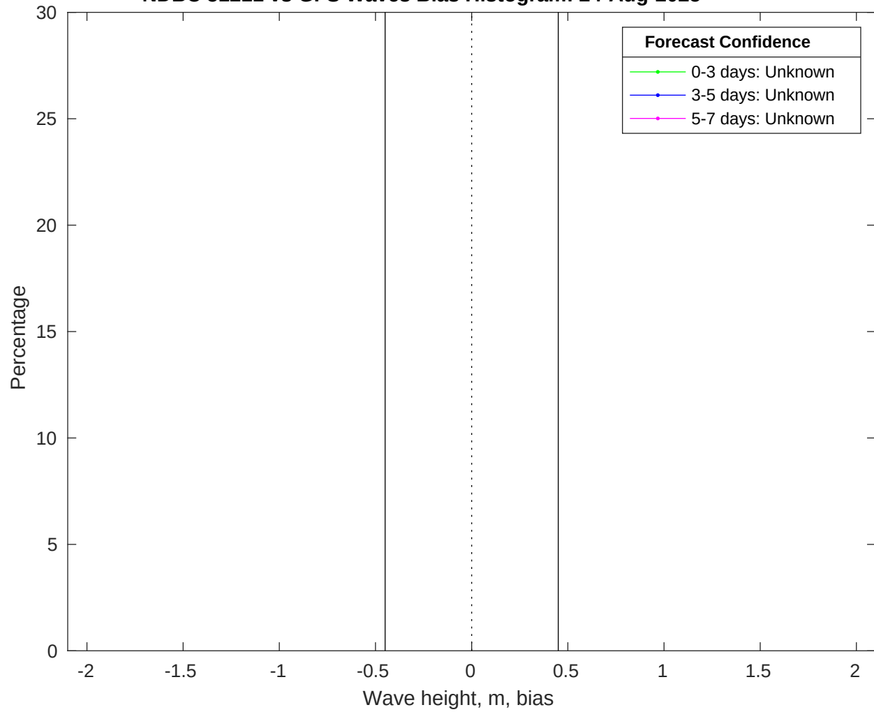
NDBC 51211 vs GFS Waves Bias Histogram: 24-Aug-2025
