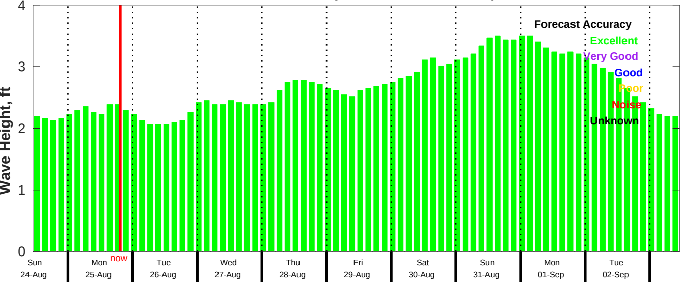
CMEMS Wave Forecast for NDBC 52211 from 23-Aug-2025 11:00:00 to 02-Sep-2025 11:00:00
