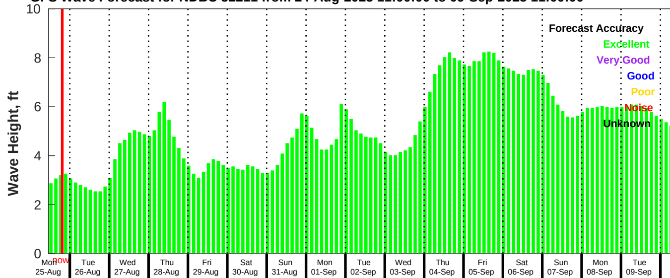
GFS Wave Forecast for NDBC 52211 from 24-Aug-2025 11:00:00 to 09-Sep-2025 11:00:00
