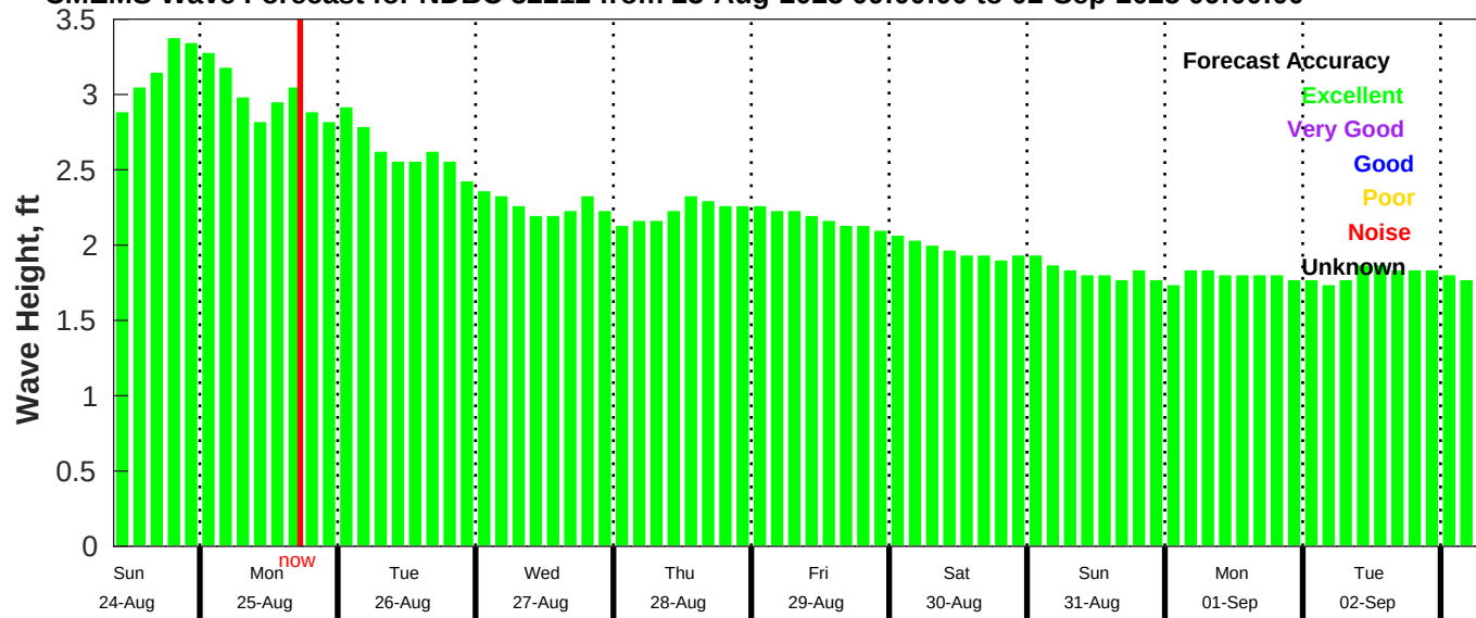
CMEMS Wave Forecast for NDBC 52212 from 23-Aug-2025 09:00:00 to 02-Sep-2025 09:00:00
