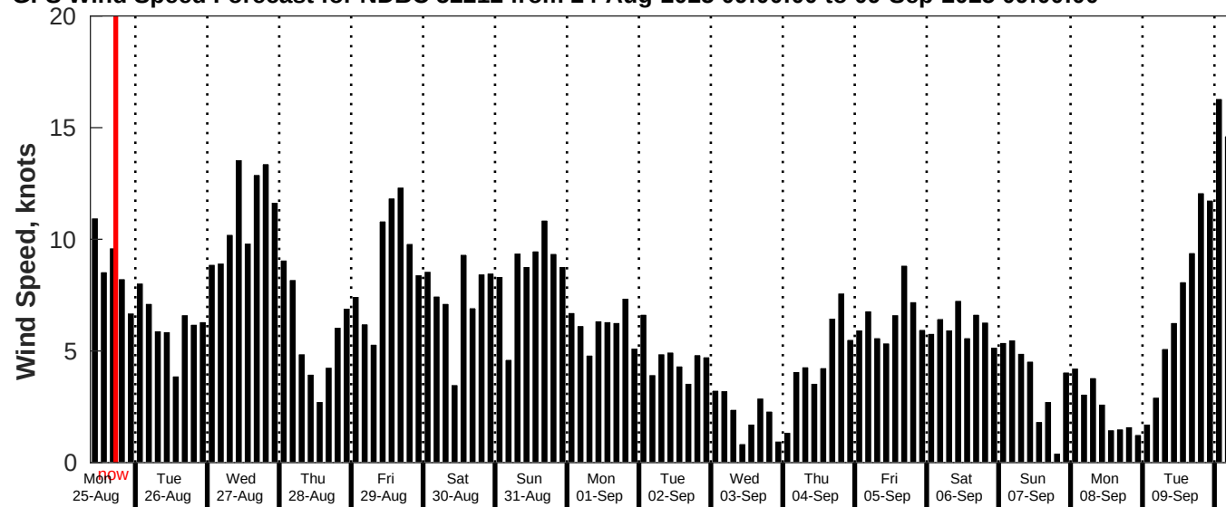
GFS Wind Speed Forecast for NDBC 52212 from 24-Aug-2025 09:00:00 to 09-Sep-2025 09:00:00
