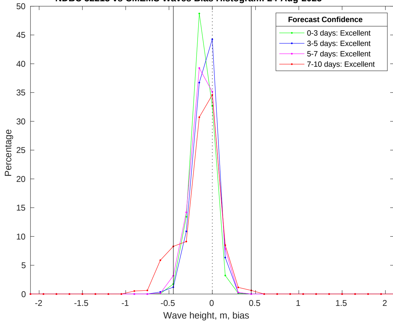
NDBC 52213 vs CMEMS Waves Bias Histogram: 24-Aug-2025
