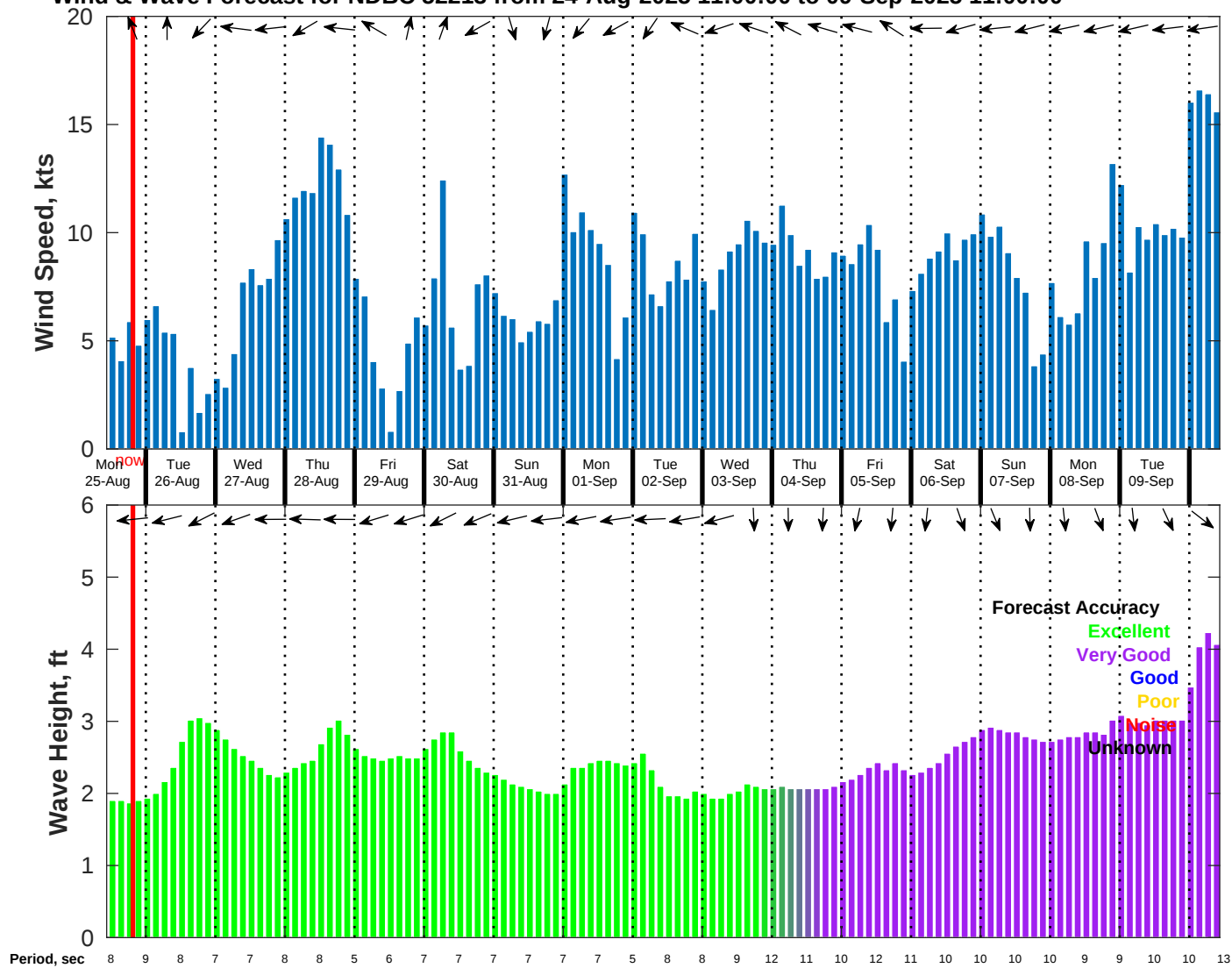
Wind & Wave Forecast for NDBC 52213 from 24-Aug-2025 11:00:00 to 09-Sep-2025 11:00:00
