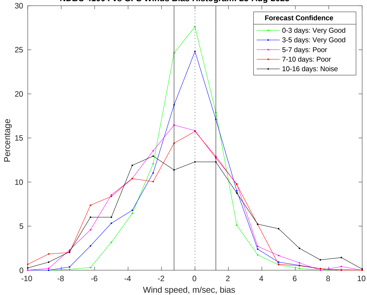
NDBC 41004 vs GFS Winds Bias Histogram: 25-Aug-2025
