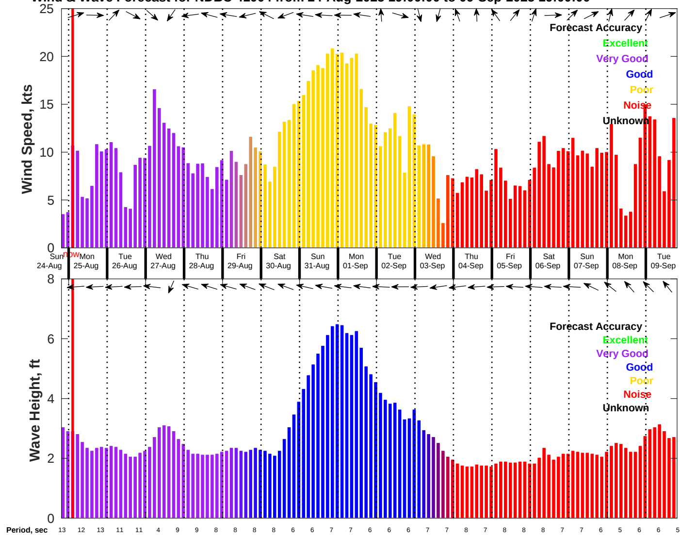
Wind & Wave Forecast for NDBC 41004 from 24-Aug-2025 19:00:00 to 09-Sep-2025 19:00:00
