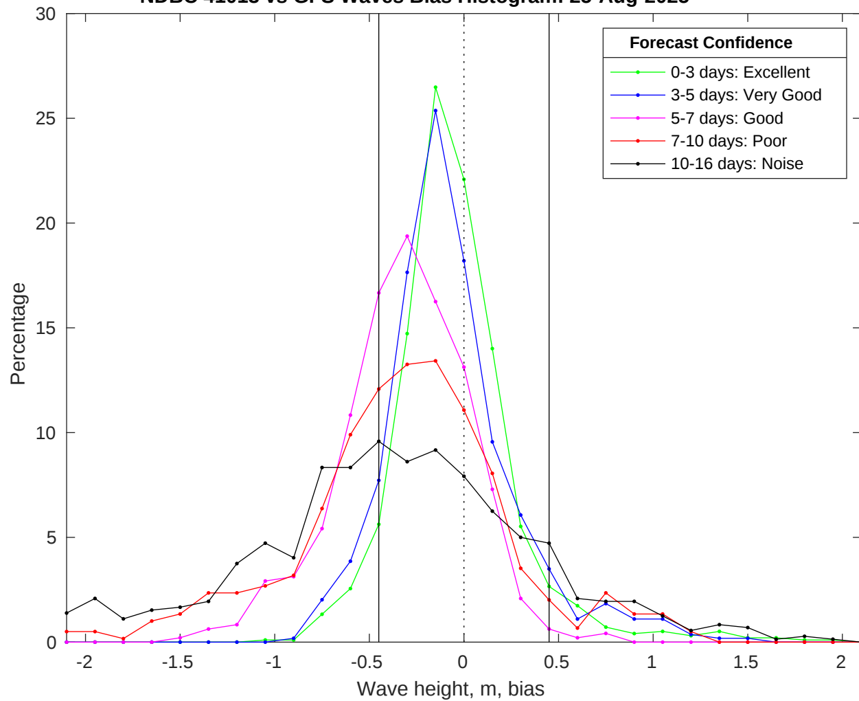
NDBC 41013 vs GFS Waves Bias Histogram: 25-Aug-2025
