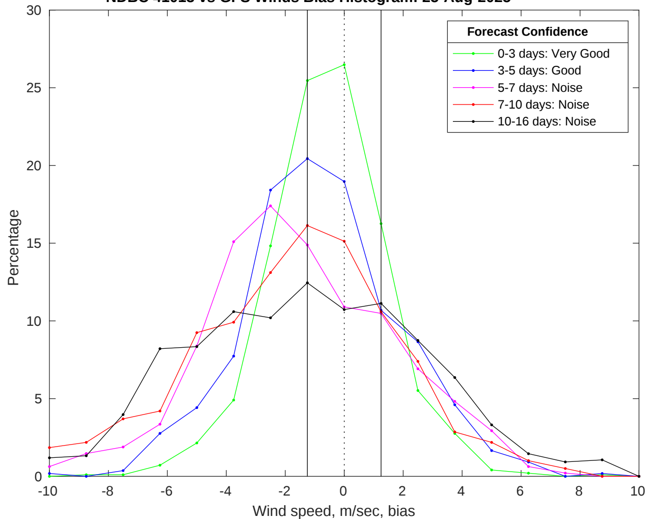
NDBC 41013 vs GFS Winds Bias Histogram: 25-Aug-2025
