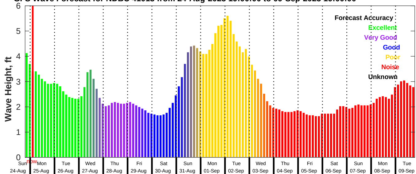
GFS Wave Forecast for NDBC 41013 from 24-Aug-2025 19:00:00 to 09-Sep-2025 19:00:00
