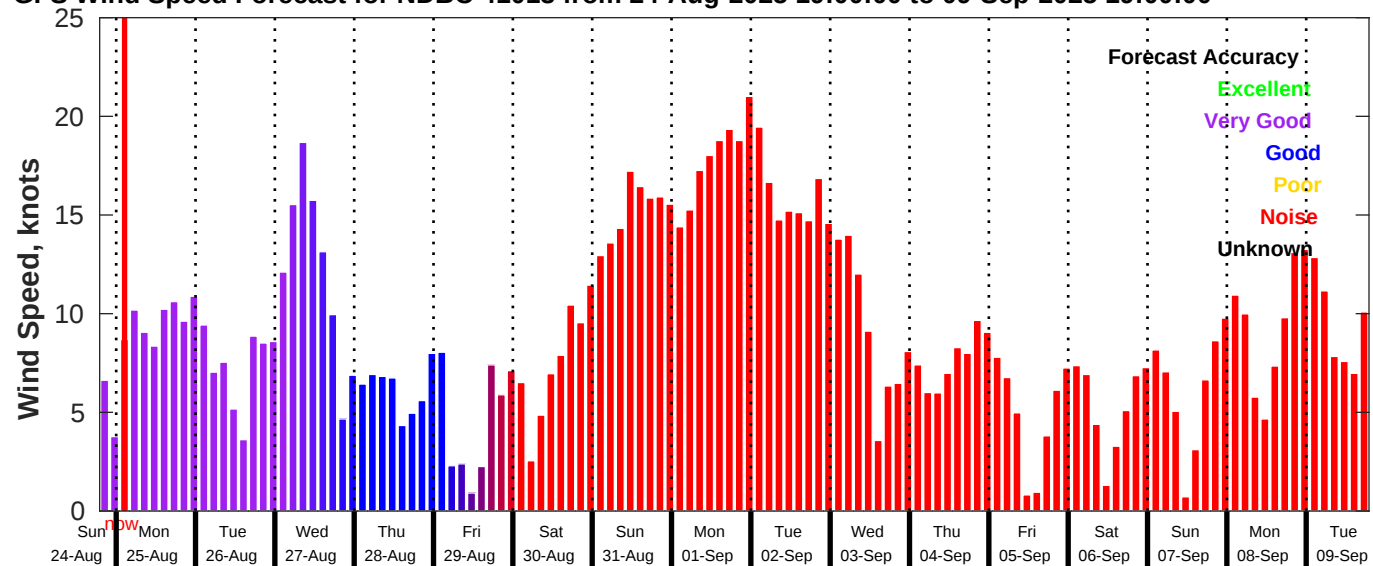
GFS Wind Speed Forecast for NDBC 41013 from 24-Aug-2025 19:00:00 to 09-Sep-2025 19:00:00
