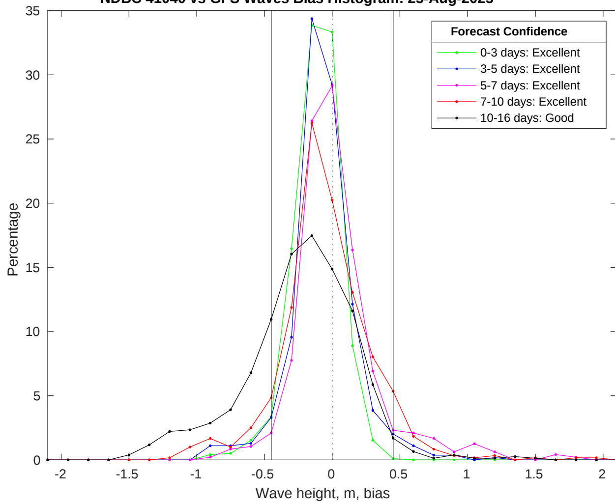
NDBC 41040 vs GFS Waves Bias Histogram: 25-Aug-2025
