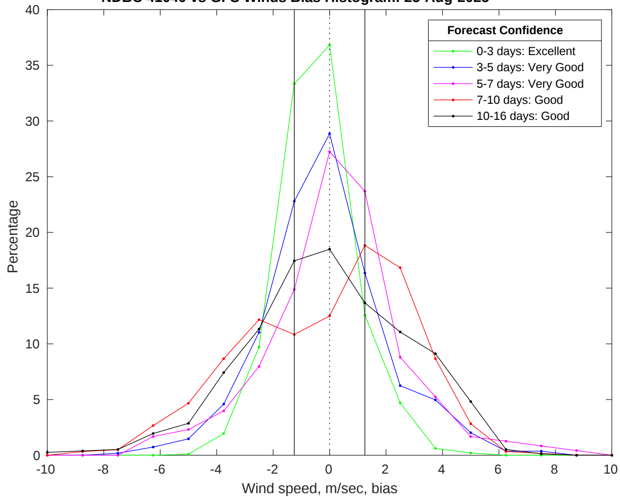
NDBC 41040 vs GFS Winds Bias Histogram: 25-Aug-2025
