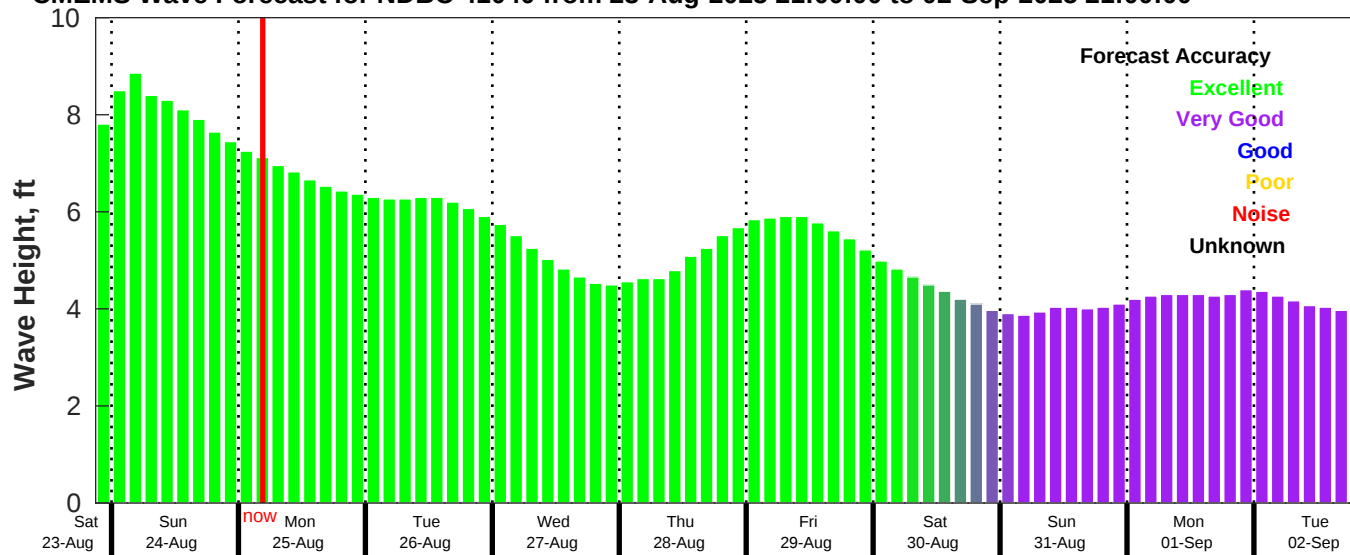
CMEMS Wave Forecast for NDBC 41040 from 23-Aug-2025 21:00:00 to 02-Sep-2025 21:00:00
