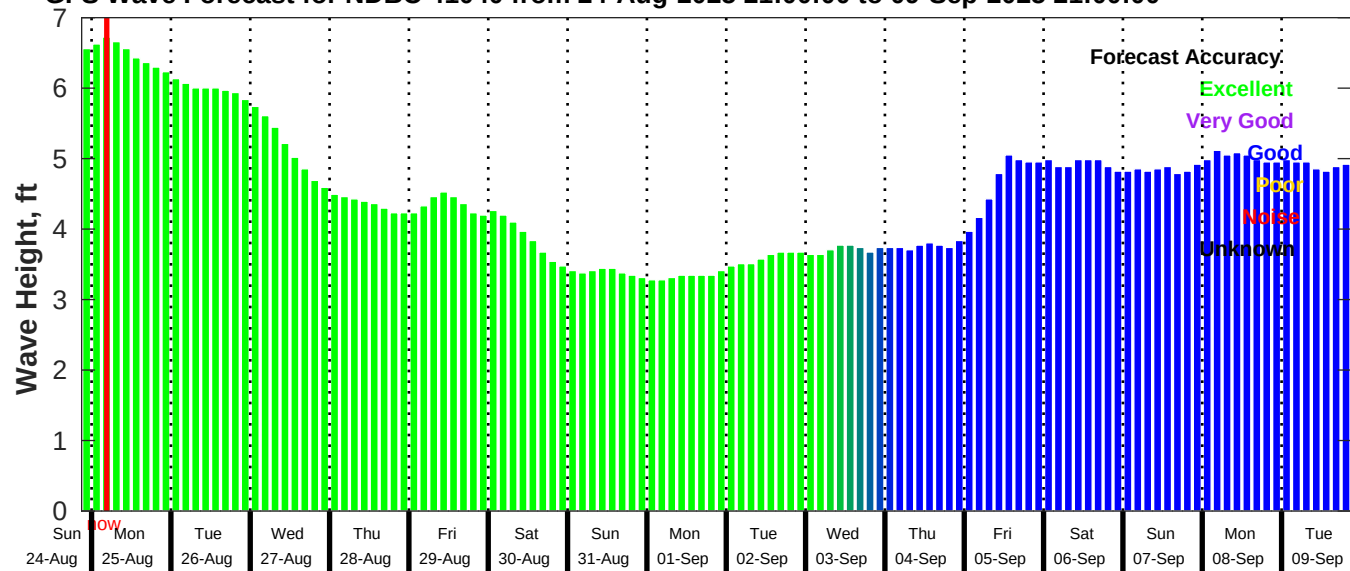
GFS Wave Forecast for NDBC 41040 from 24-Aug-2025 21:00:00 to 09-Sep-2025 21:00:00
