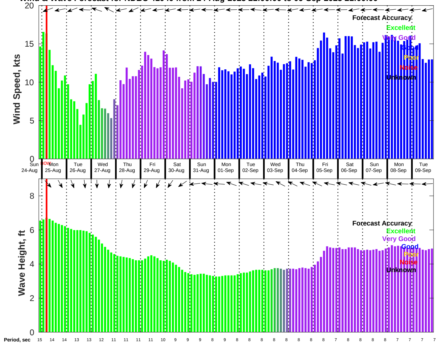
Wind & Wave Forecast for NDBC 41040 from 24-Aug-2025 21:00:00 to 09-Sep-2025 21:00:00
