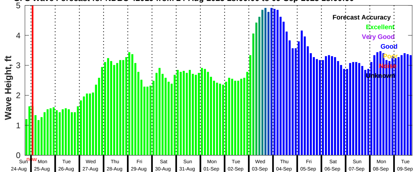
GFS Wave Forecast for NDBC 42019 from 24-Aug-2025 18:00:00 to 09-Sep-2025 18:00:00
