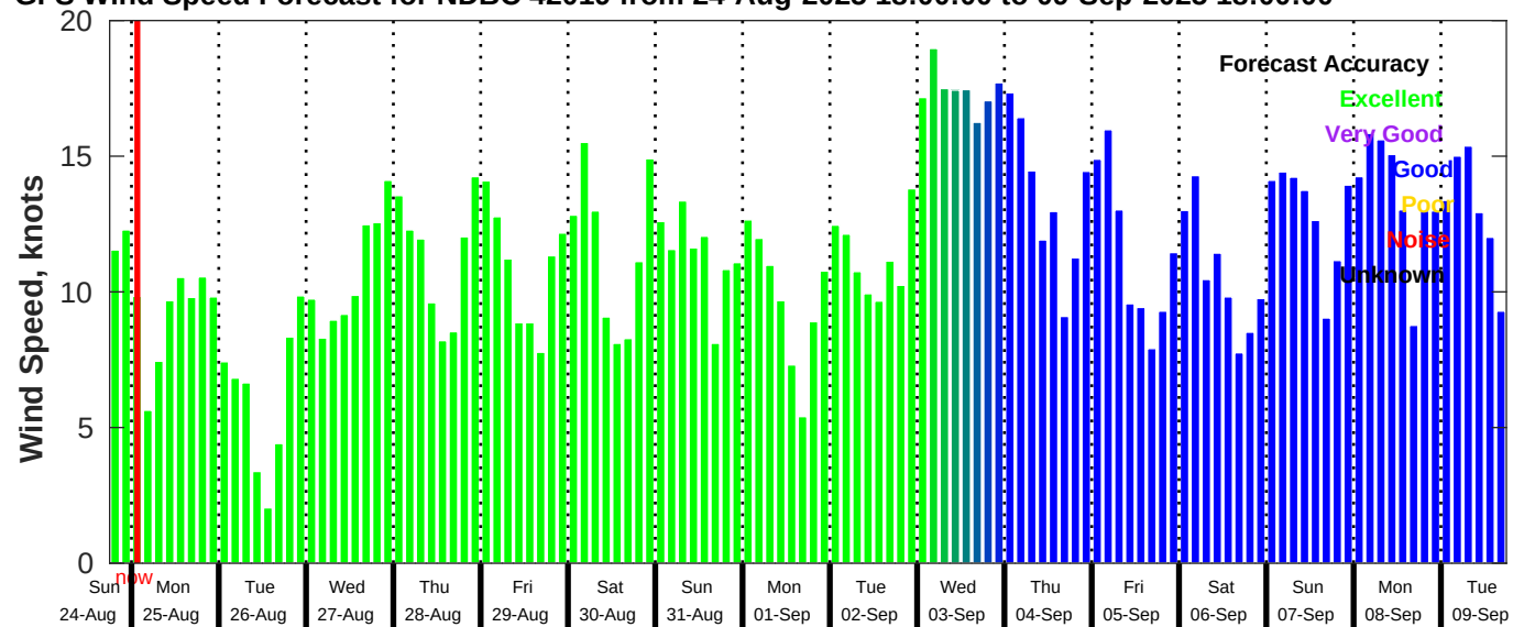
GFS Wind Speed Forecast for NDBC 42019 from 24-Aug-2025 18:00:00 to 09-Sep-2025 18:00:00
