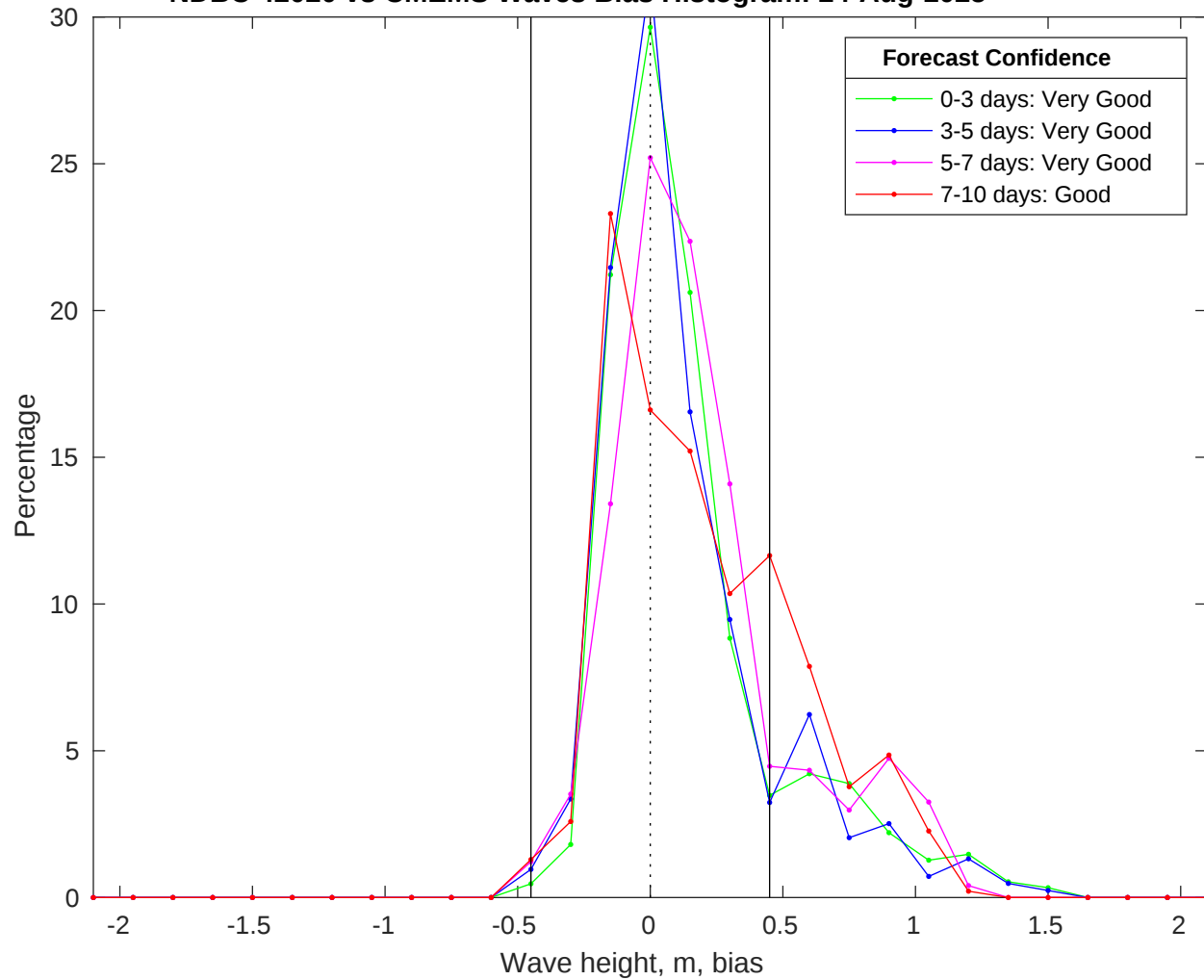
NDBC 42020 vs CMEMS Waves Bias Histogram: 24-Aug-2025
