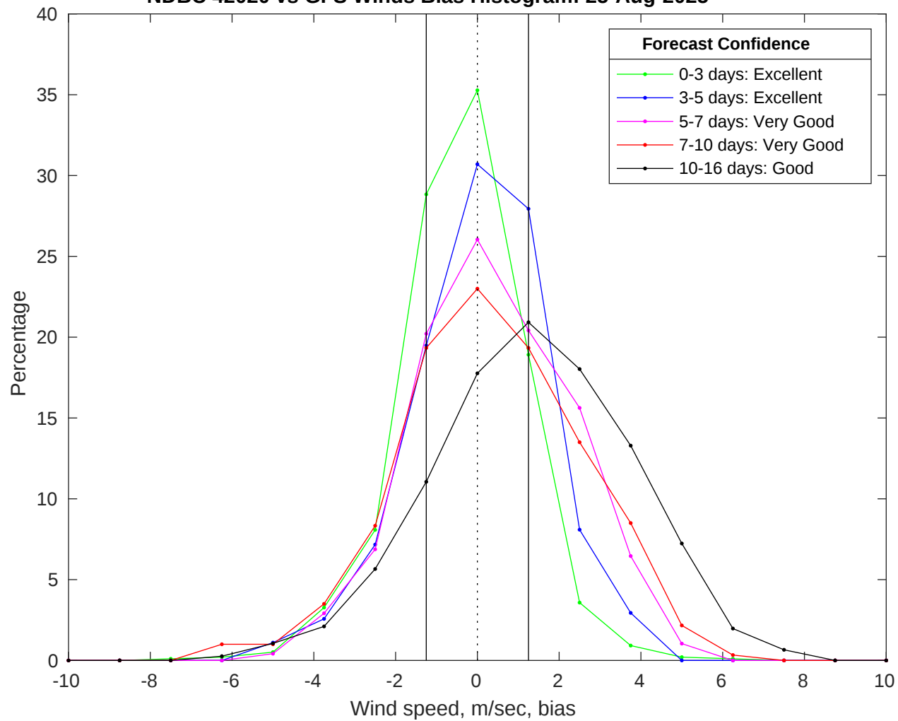
NDBC 42020 vs GFS Winds Bias Histogram: 25-Aug-2025
