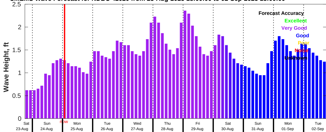
CMEMS Wave Forecast for NDBC 42020 from 23-Aug-2025 18:00:00 to 02-Sep-2025 18:00:00
