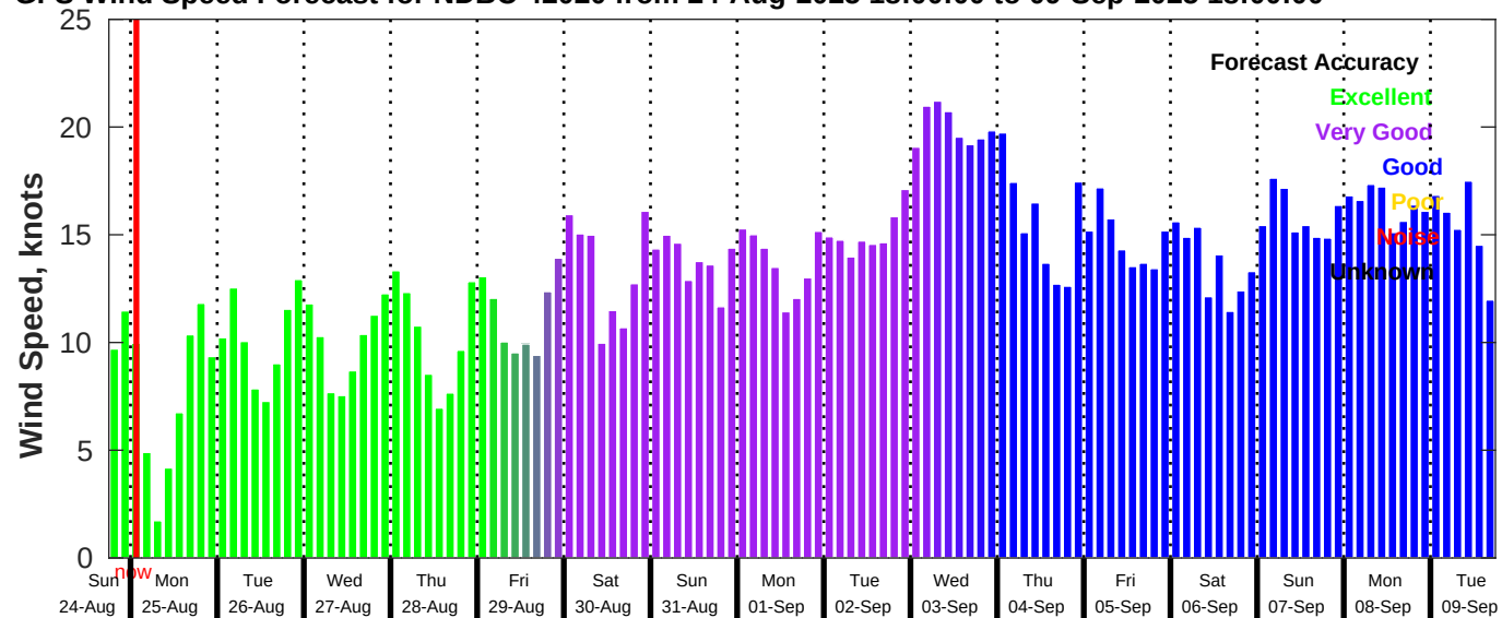
GFS Wind Speed Forecast for NDBC 42020 from 24-Aug-2025 18:00:00 to 09-Sep-2025 18:00:00
