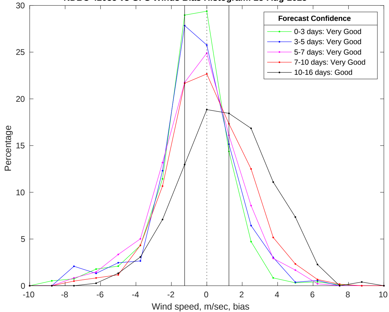
NDBC 42035 vs GFS Winds Bias Histogram: 25-Aug-2025
