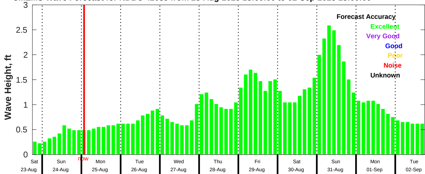
CMEMS Wave Forecast for NDBC 42035 from 23-Aug-2025 18:00:00 to 02-Sep-2025 18:00:00
