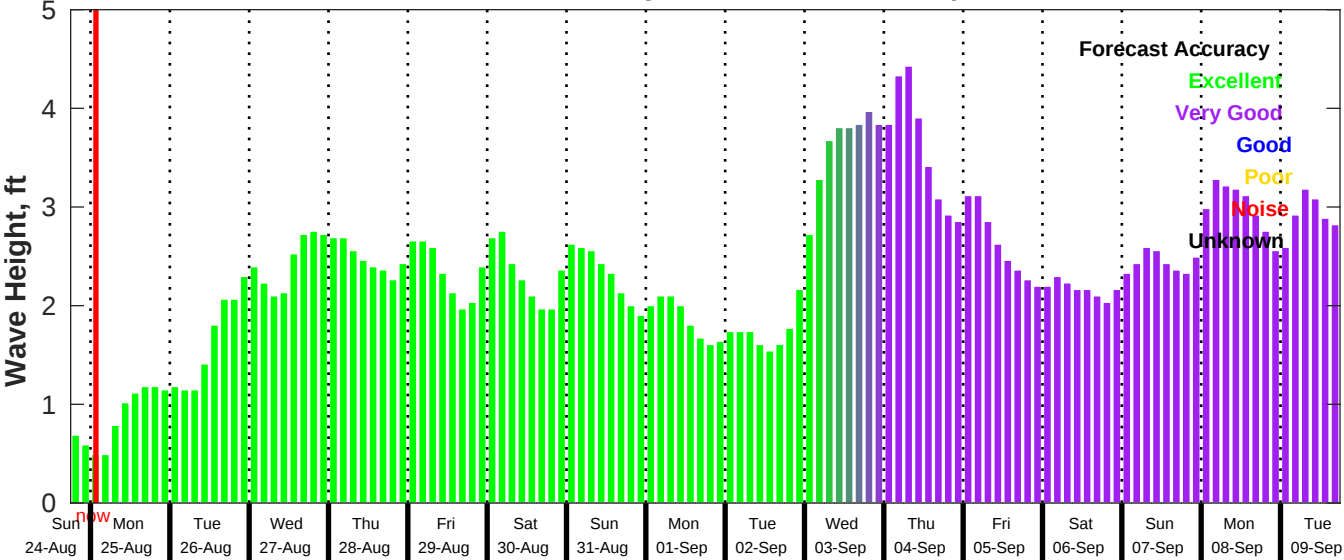
GFS Wave Forecast for NDBC 42035 from 24-Aug-2025 18:00:00 to 09-Sep-2025 18:00:00
