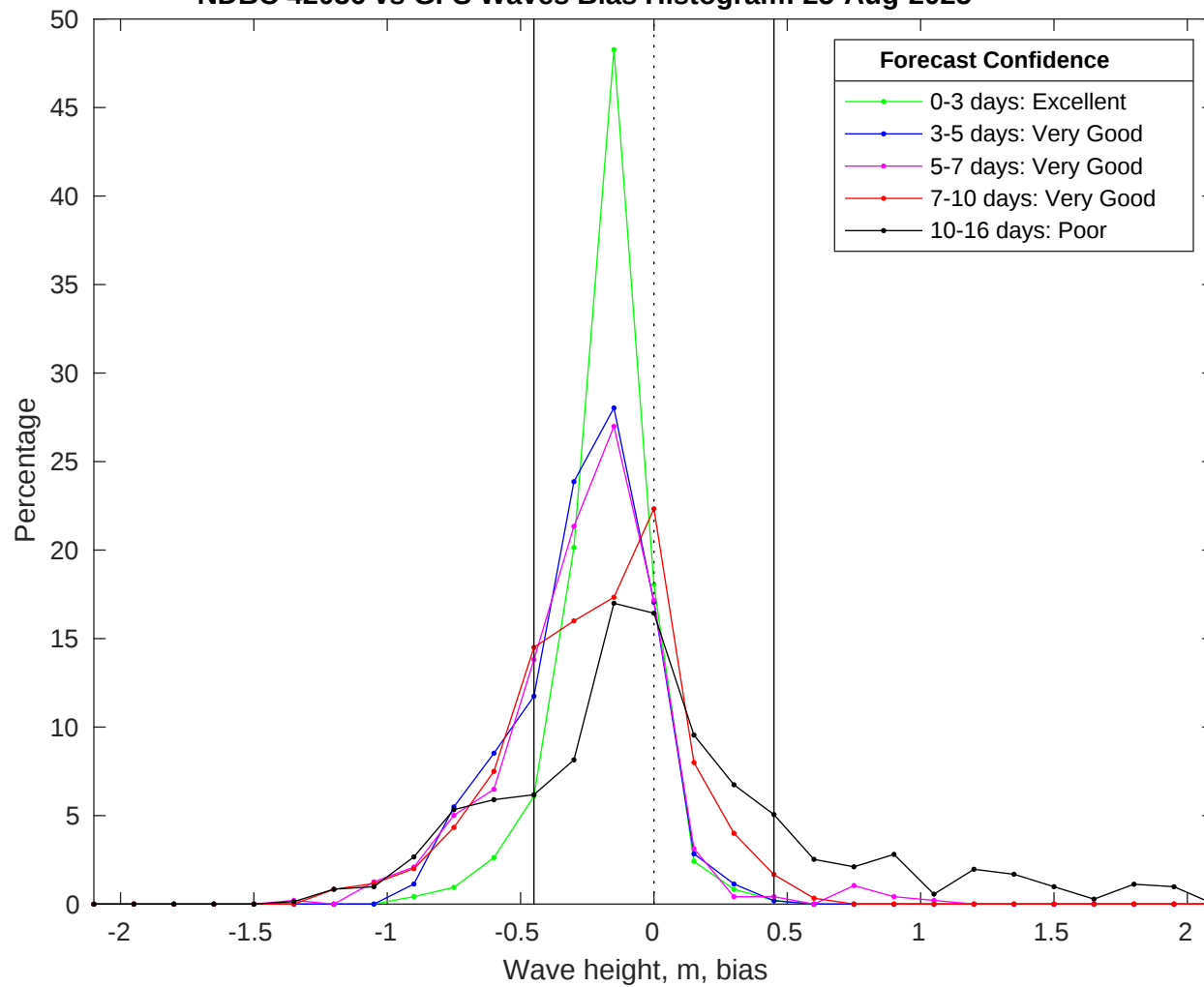
NDBC 42036 vs GFS Waves Bias Histogram: 25-Aug-2025
