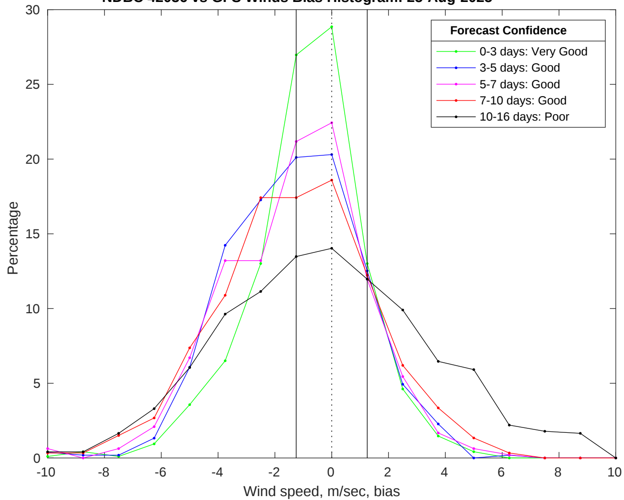
NDBC 42036 vs GFS Winds Bias Histogram: 25-Aug-2025
