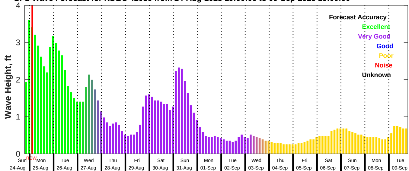
GFS Wave Forecast for NDBC 42036 from 24-Aug-2025 19:00:00 to 09-Sep-2025 19:00:00
