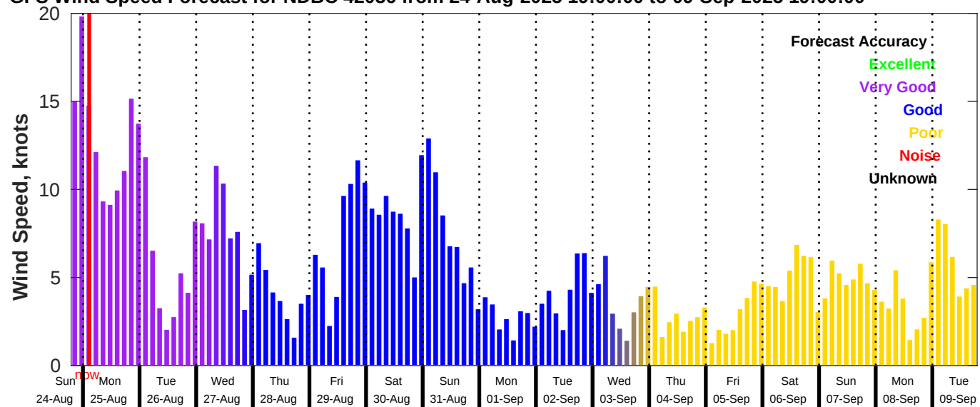
GFS Wind Speed Forecast for NDBC 42036 from 24-Aug-2025 19:00:00 to 09-Sep-2025 19:00:00
