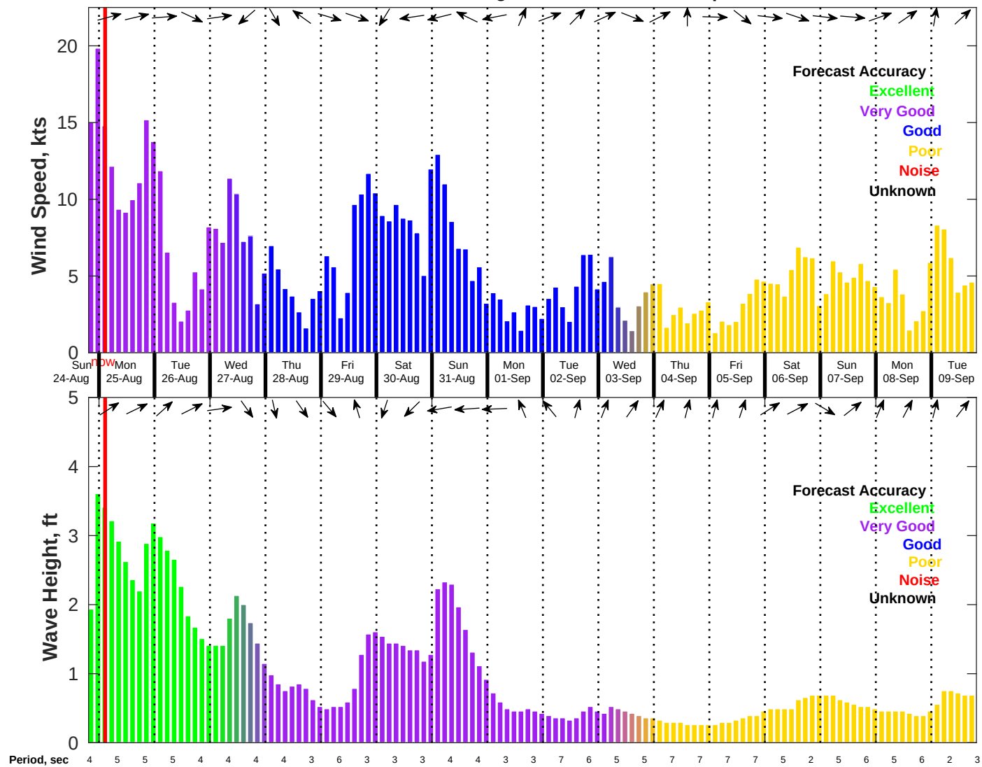
Wind & Wave Forecast for NDBC 42036 from 24-Aug-2025 19:00:00 to 09-Sep-2025 19:00:00
