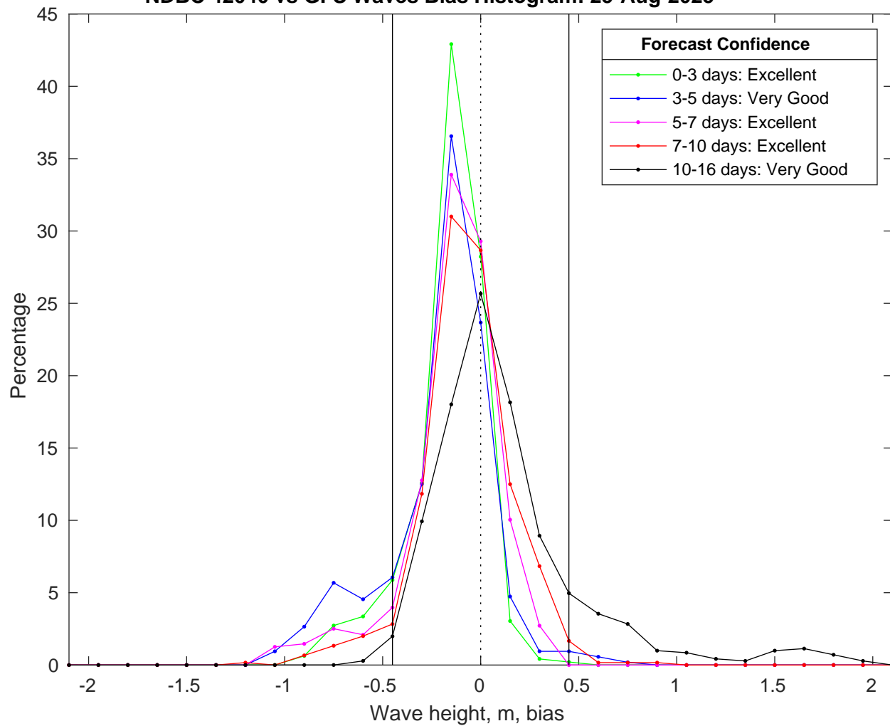
NDBC 42040 vs GFS Waves Bias Histogram: 25-Aug-2025
