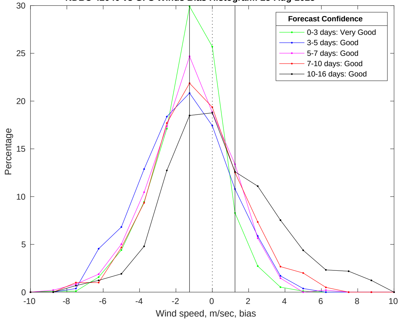
NDBC 42040 vs GFS Winds Bias Histogram: 25-Aug-2025
