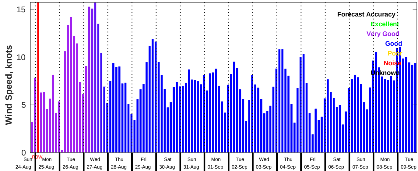
GFS Wind Speed Forecast for NDBC 42040 from 24-Aug-2025 19:00:00 to 09-Sep-2025 19:00:00
